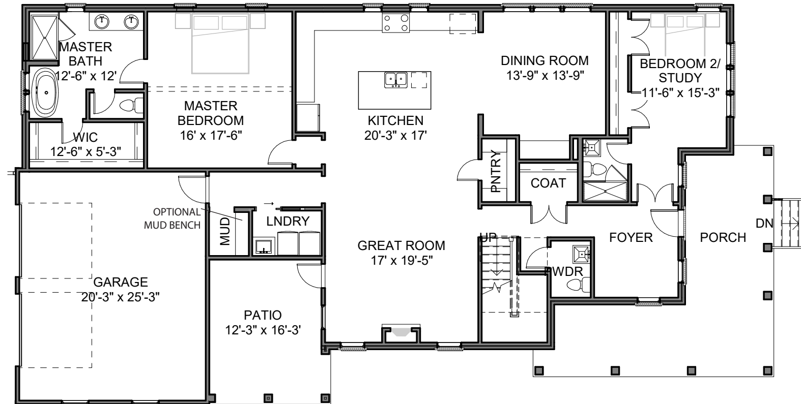
1ST AND 2ND FLOOR PLANS
