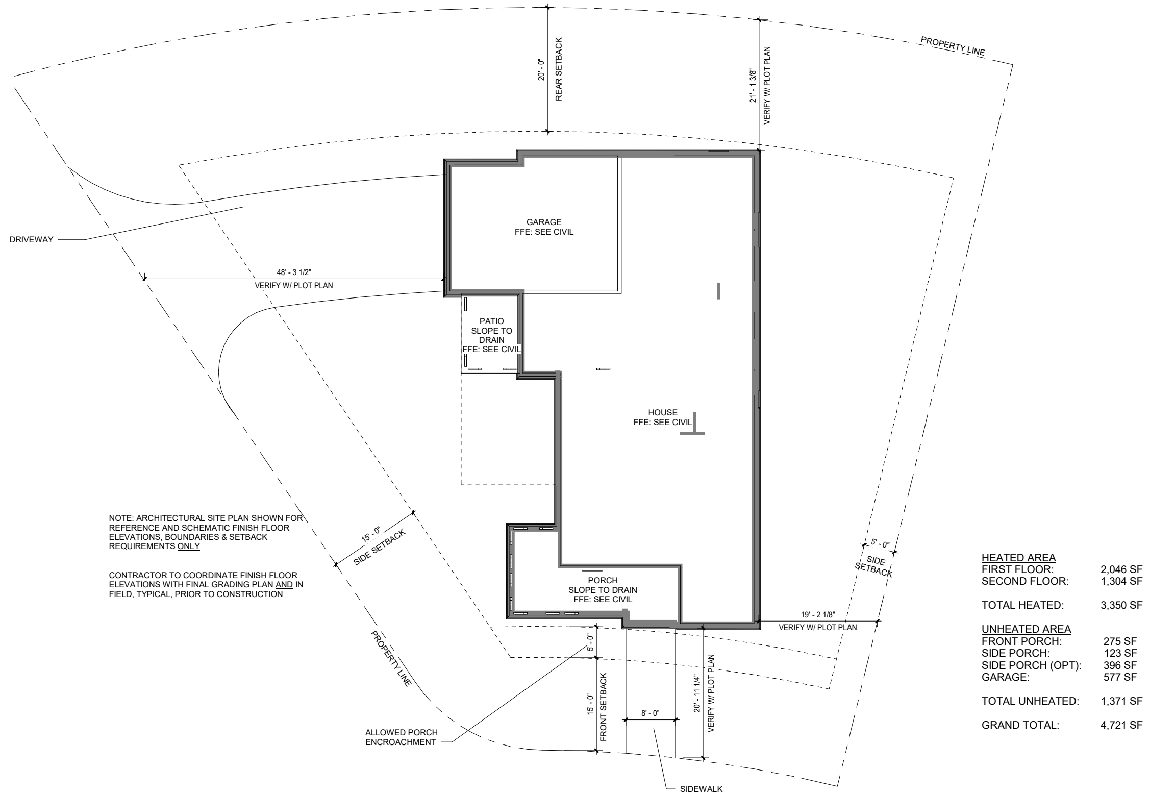
SITE PLAN
