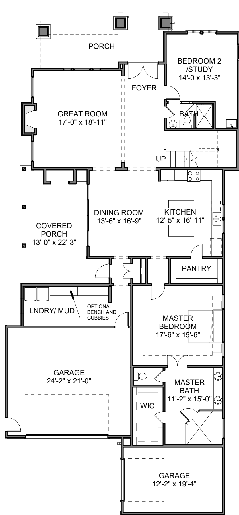
1ST AND 2ND FLOOR PLANS
